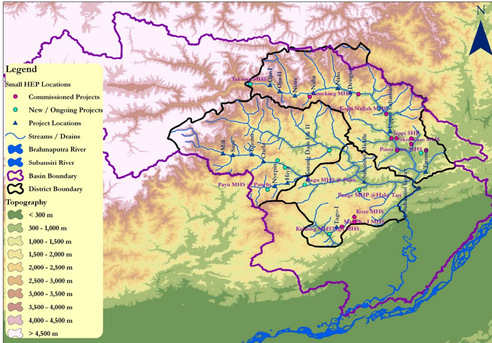
Figure 3.1: Location, Physiography & Topography of the Projects
