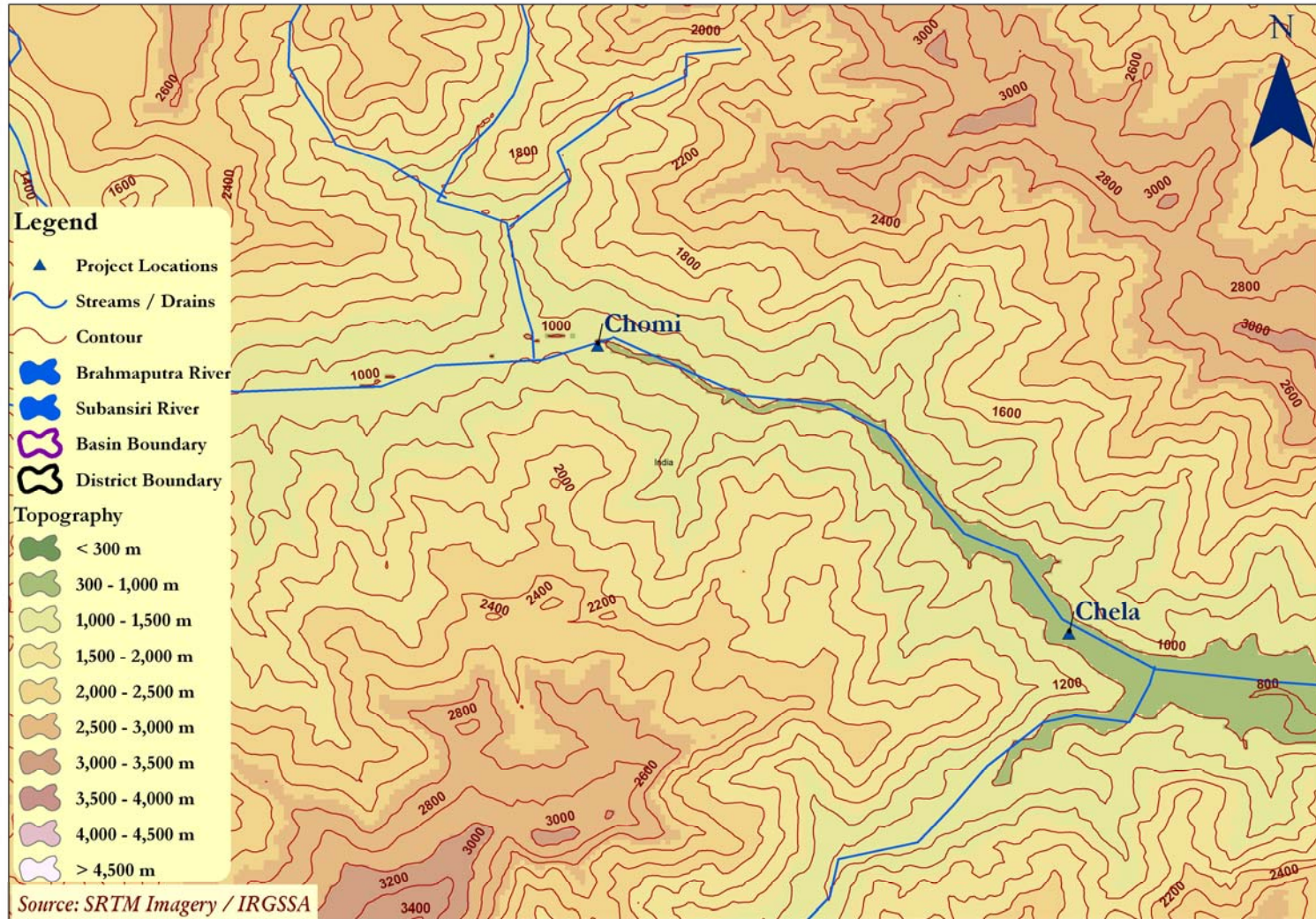
Figure 3.10: Chomi & Chela HEPs-Location, Physiography & Topography of the Projects
