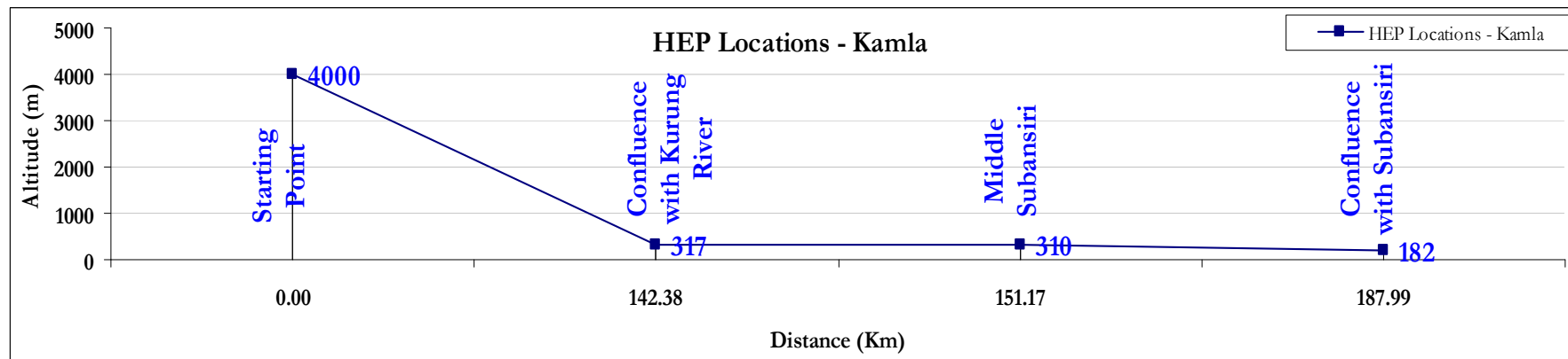
Figure 8.2: Proposed Cascade Development of HEP on Kamla River
