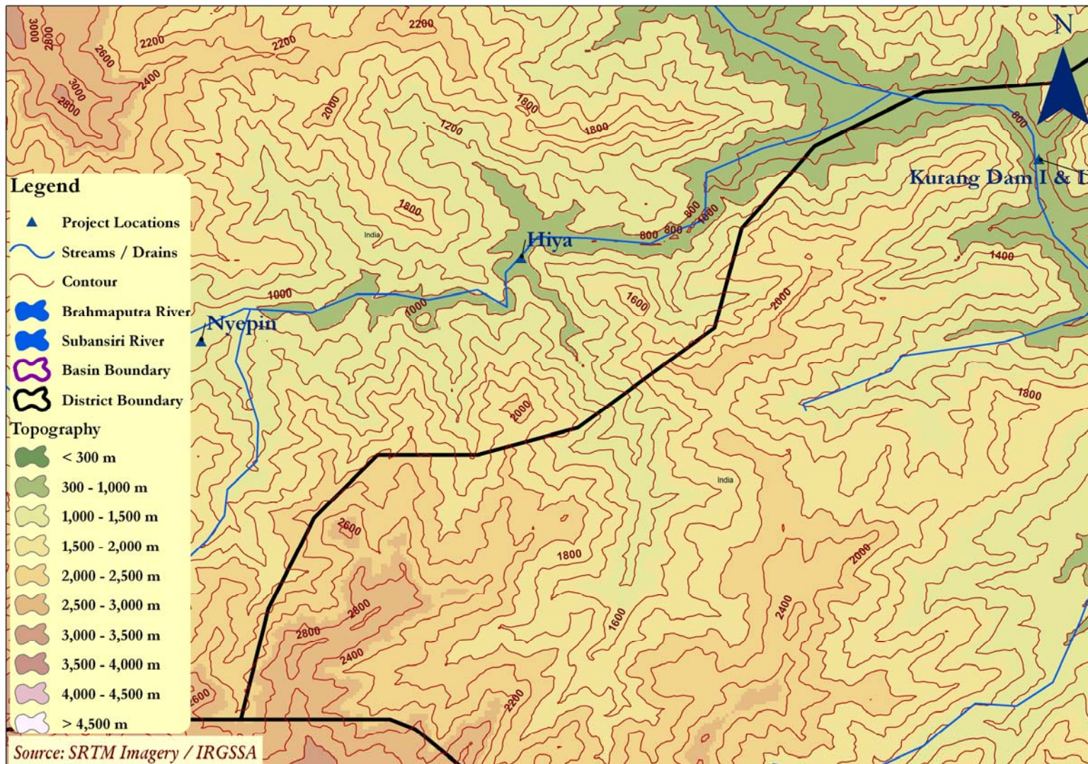
Figure 3.9: Nyepin, Hiya & Kurang I & II HEPs- Location, Physiography & Topography of the Projects
