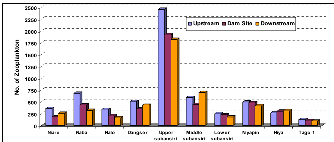
Figure 7.24: Numbers of Zooplankton recorded (organism/1)
