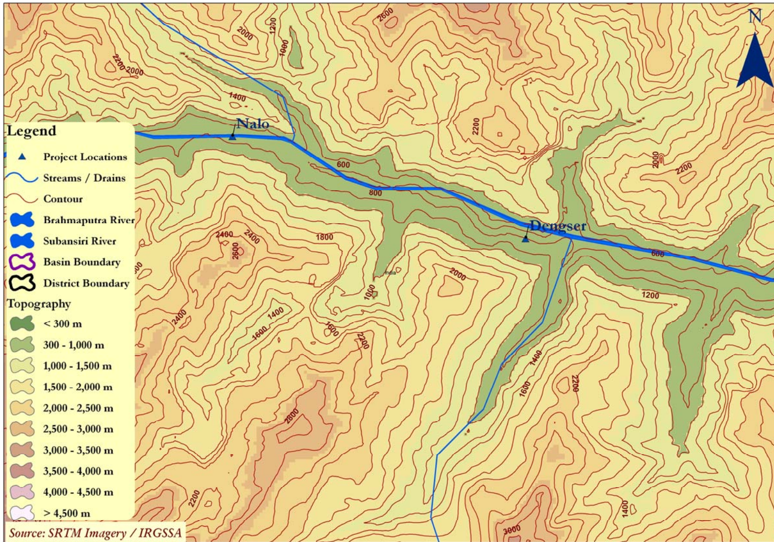
Figure 3.4: Nalo and Dengser HEPs- Location, Physiography & Topography of the Projects
